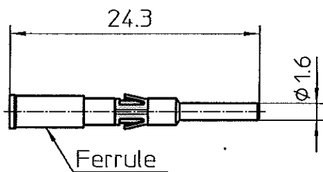
Pin contact
