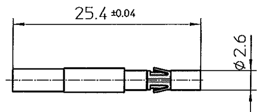
Socket contact (After Assembly)
